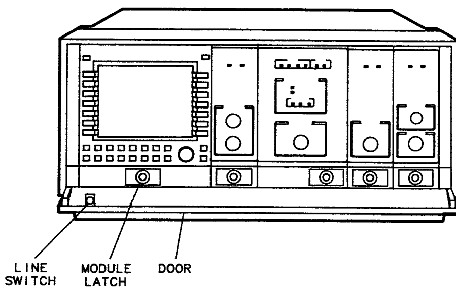
Figure 2-2. Module Installation
